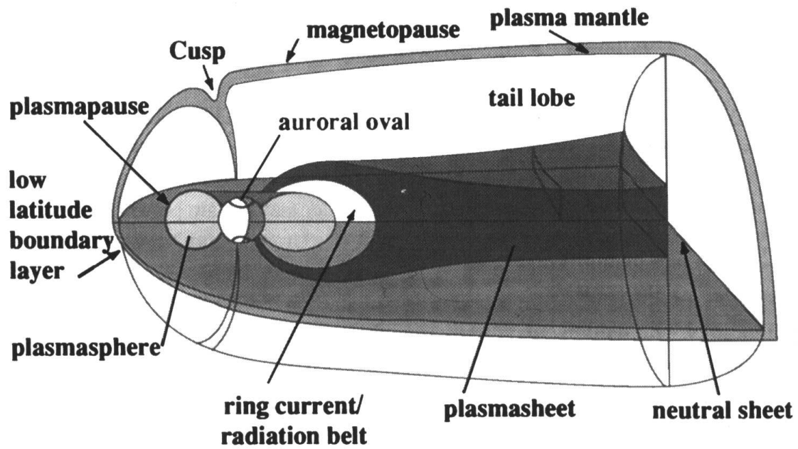
Figure 14.1: Schematic illustration of Earth's magnetotail, emphasizing the different plasma regions [Cravens, 1997]. Note the cusps, plasma mantle, tail lobes, plasmashet, neutral sheet, ring current, radiation belts, plasmasphere, and auroral ovals.
